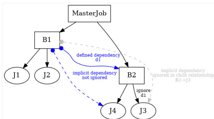
Figure 15.19: Example of Ignored Dependencies
