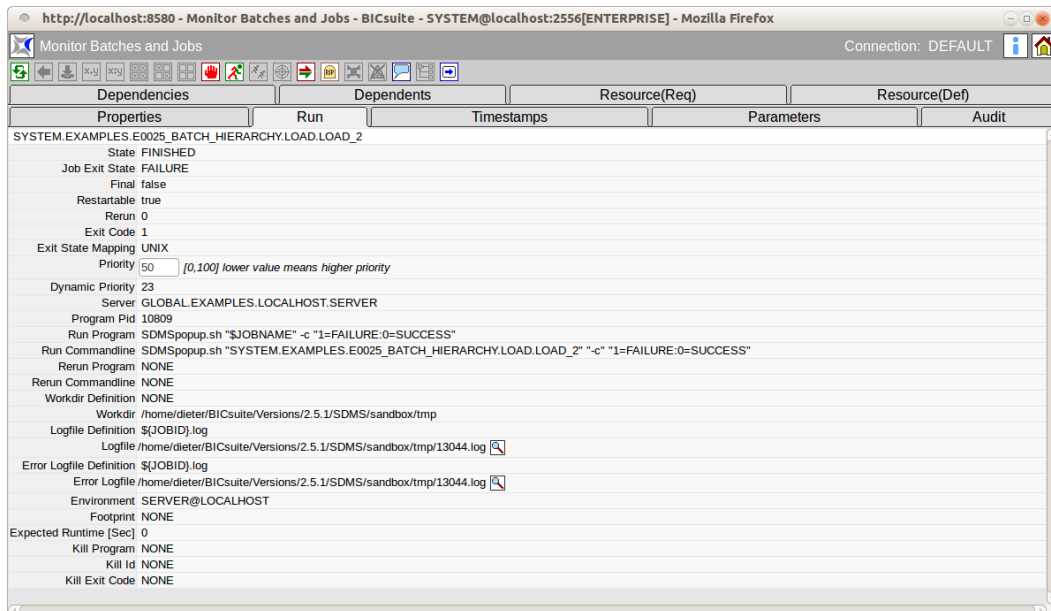
Figure 23.10: Batch und Job Run information
