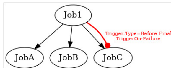
Figure 15.39: Example of a Before Final Trigger
