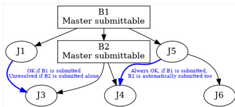
Figure 15.24: Example for Unresolved Handling
