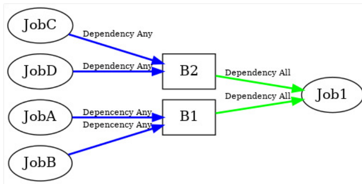
Figure 15.22: Example of Dependency Modes
