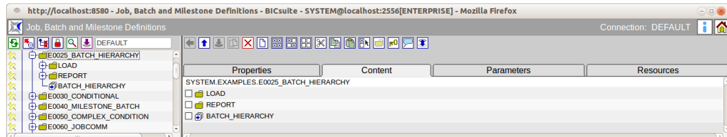
Figure 15.6: Folder content
