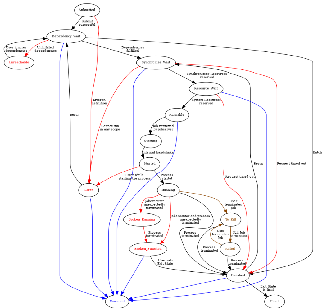
Figure 23.3: State chart for batches and jobs
