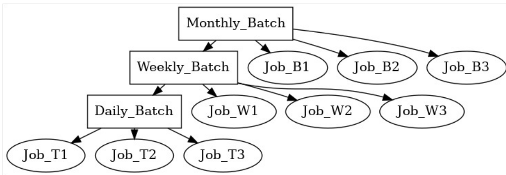
Figure 15.11: Examples of batches
