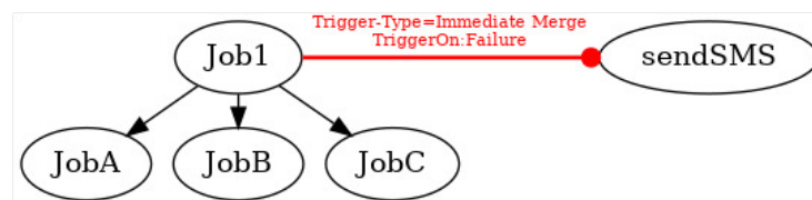
Figure 15.37: Example of an Immediate Merge trigger
