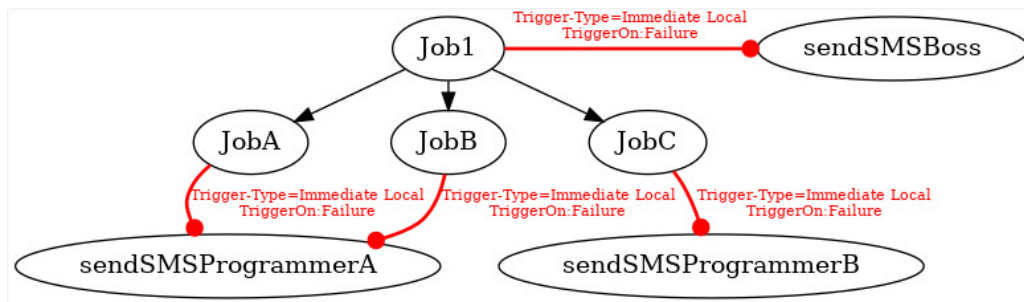
Figure 15.38: Example of an Immediate Local trigger
