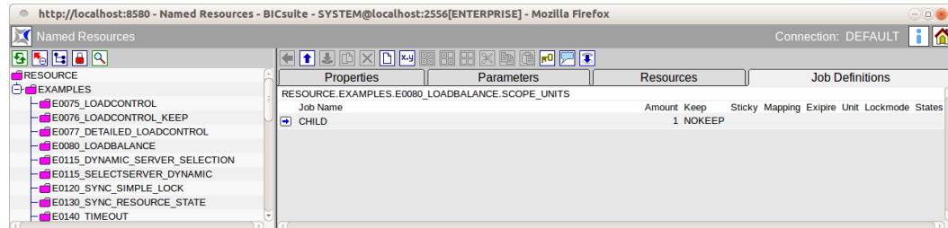
Figure 11.8: Named Resources; Job Definitions tab
