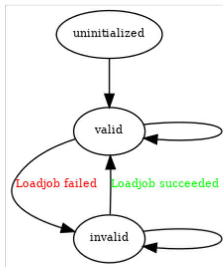
Figure 8.3: State chart for a resource
