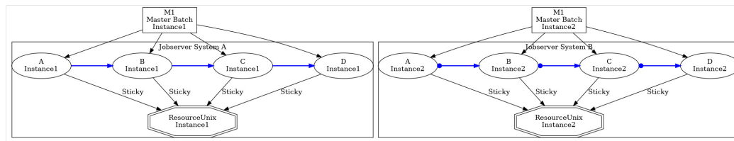
Figure 15.29: Example of load distribution with Sticky Handling
