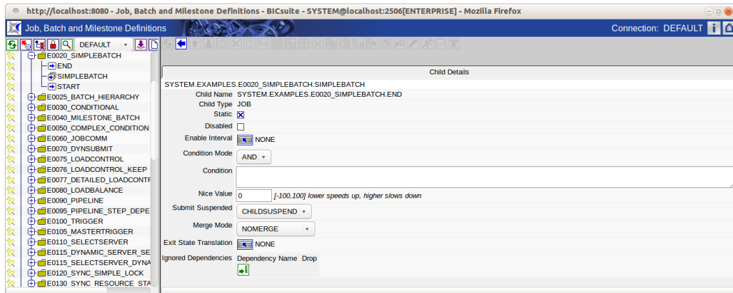
Figure 15.16: Batches and Jobs; Child Details tab
