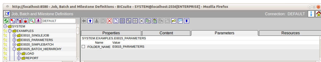
Figure 15.8: Folder parameters
