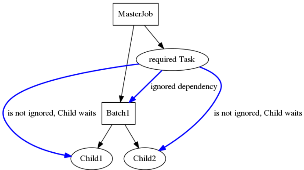
Figure 22.15: Example of a Job Only Ignore
