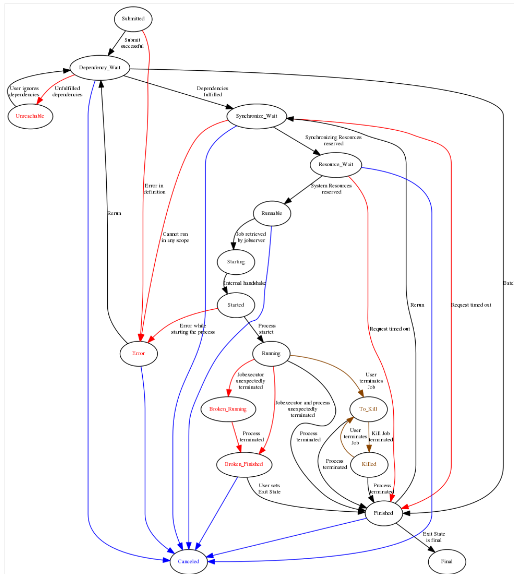
Figure 22.3: State chart for batches and jobs
