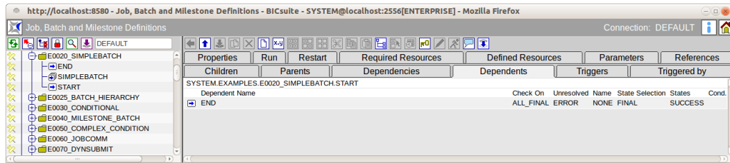
Figure 15.25: Batches and Jobs; Dependents tab
