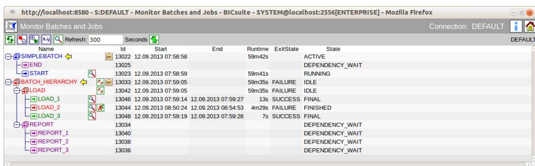
Figure 23.1: Search Running Jobs
