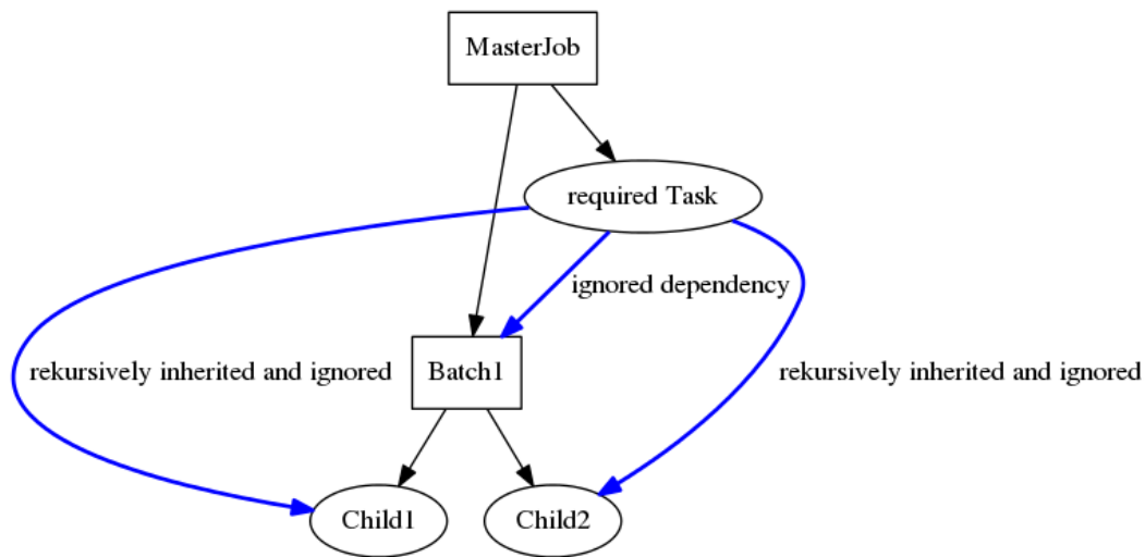
Figure 22.14: Example of a Recursive Ignore
