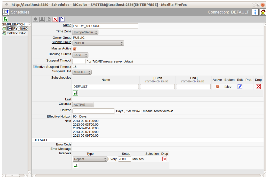
Figure 19.2: Time Scheduling Navigator
