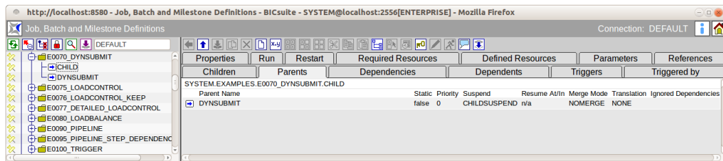
Figure 15.20: Batches and Jobs; Parents tab
