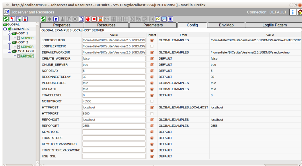
Figure 14.11: Jobserver and scope configuration
