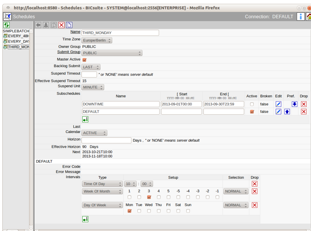
Figure 19.3: Time Scheduling Editor
