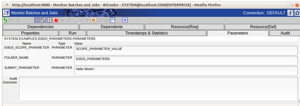
Figure 22.21: Batch and job parameters
