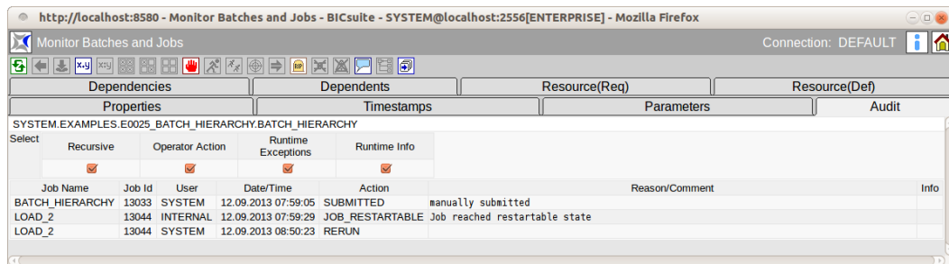
Figure 22.22: Batch and job auditing
