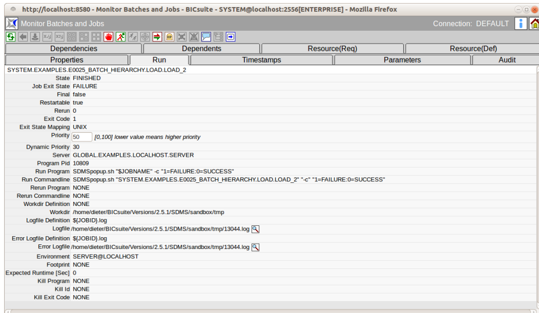
Figure 22.7: Details mask for jobs
