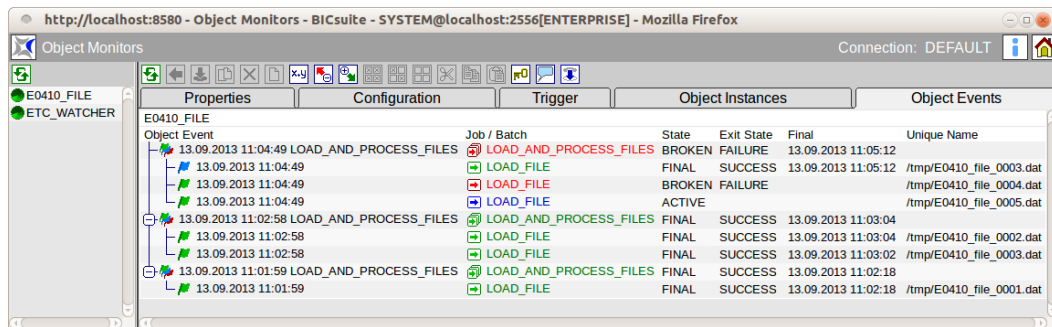
Figure 26.9: Object Monitoring Object Events
