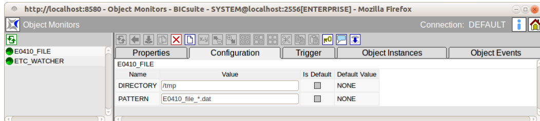
Figure 26.5: Object Monitoring configuration
