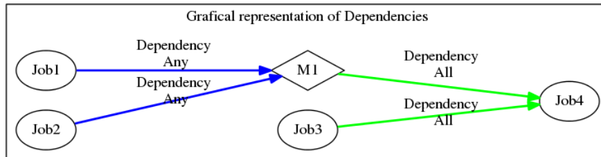
Figure 1.38: Legend for the graphical representation of dependency relationships
